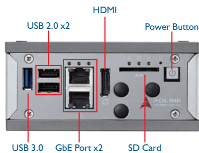
■ Front view of MXE-200/200i
