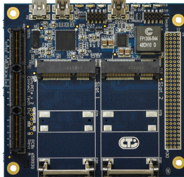
Part #: ADG044
