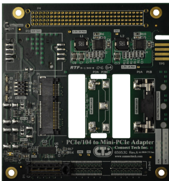
Part #: ADG028
